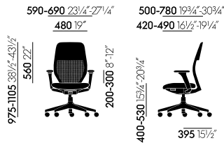
ACX Mesh with 3D armrests
