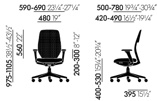
ACX Soft with 3D armrests
