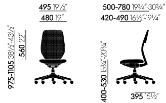
ACX Soft without armrests
