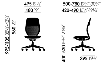
ACX Mesh without armrests
