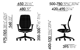
ACX Soft with height-adjustable armrests
