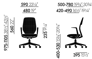
ACX Soft with fixed armrests
