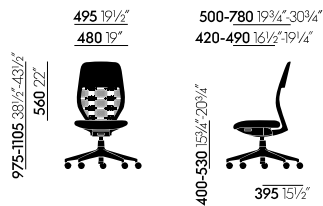
ACX Light without armrests
