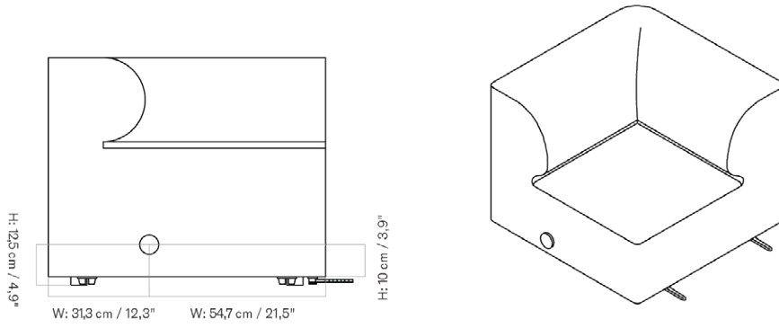
Eave 86 Open End Left
