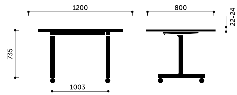
u-Connect 3490-27
