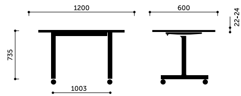
u-Connect 3490-54
