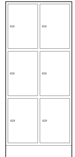
SDF8/19 1932 x 800 x 372
